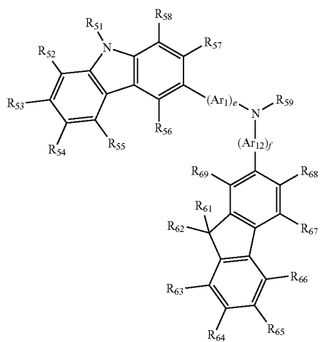
Formula 1
