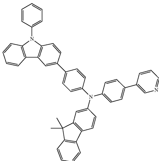
COMPOUND 14
