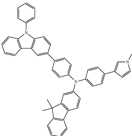
COMPOUND 31
