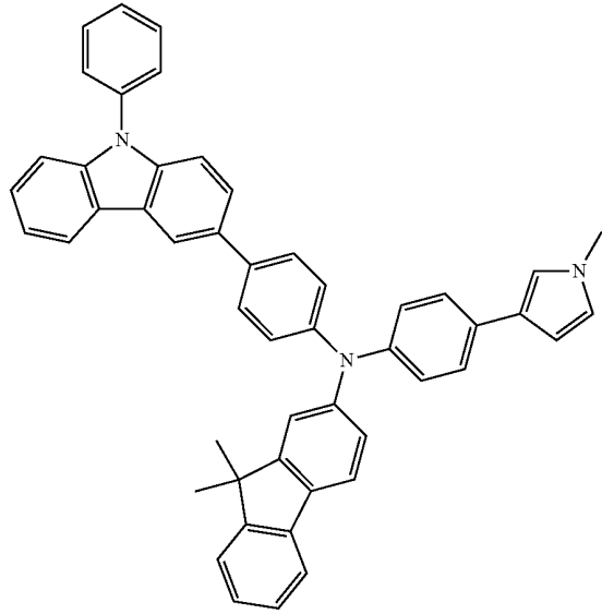
COMPOUND 31
