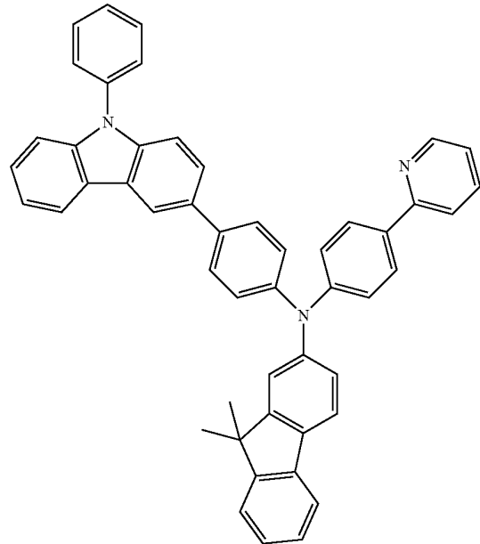
COMPOUND 35
