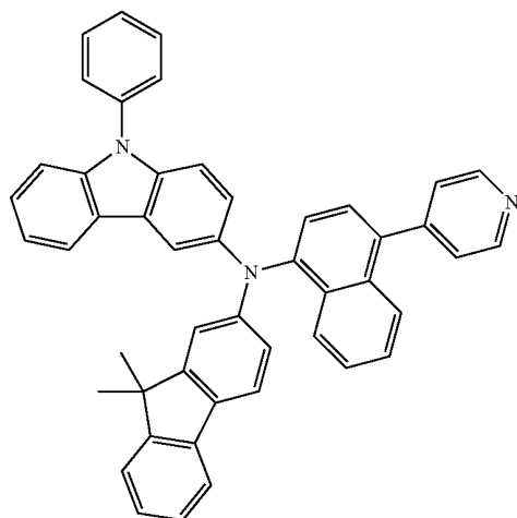
COMPOUND 8
