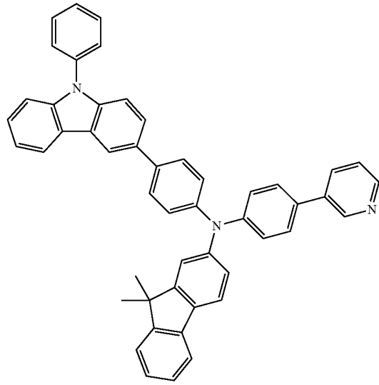
COMPOUND 14
