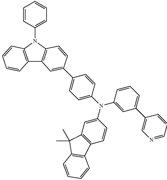
COMPOUND 16
