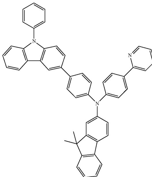
COMPOUND 35
