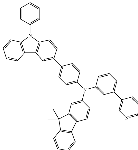
COMPOUND 16
