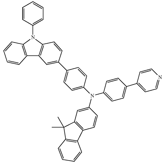
COMPOUND 15
