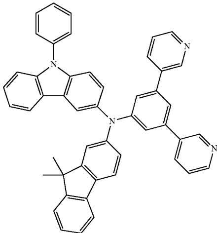
COMPOUND 8
