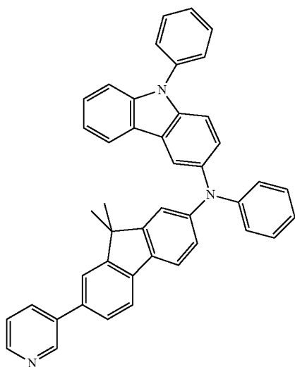
COMPOUND 20
