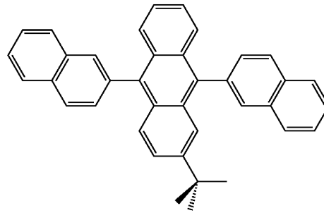
TBADN
