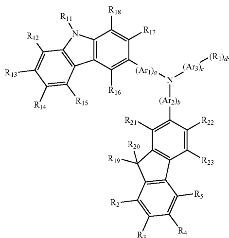
Formula 2
