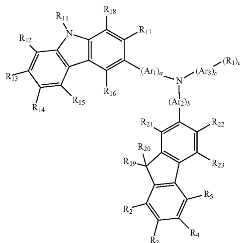
Formula 2
