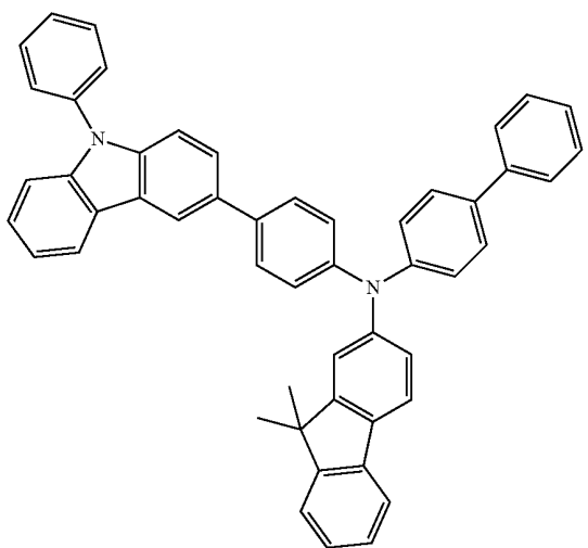
Compound 301
