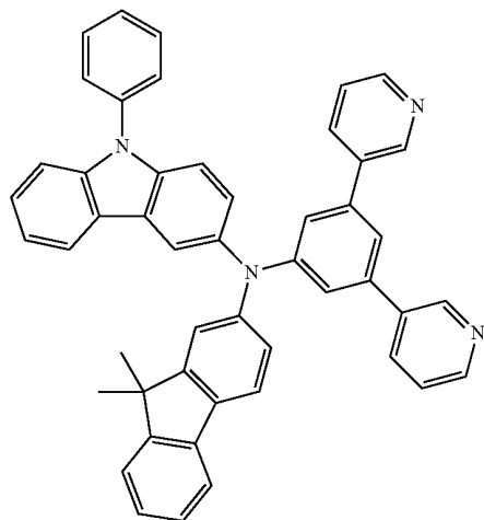
COMPOUND 14
