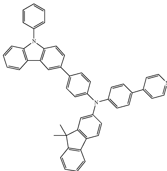
COMPOUND 15
